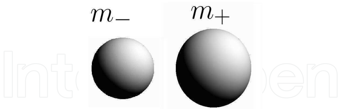
Fig. 3. Light and heavy fermion species of Lagrangian 25. Adapted from Ref. (Hernández Ortíz, 2011).
