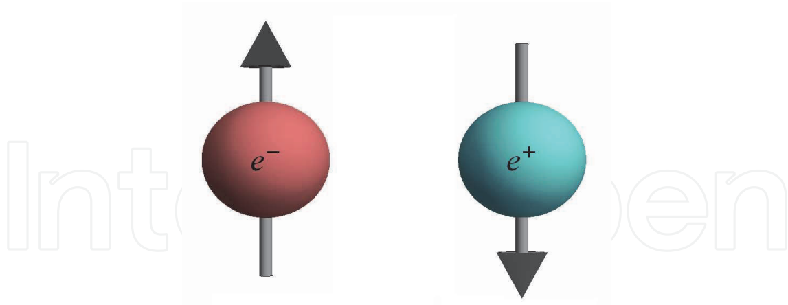
Fig. 1. The particle spectrum of solutions to the Dirac equation in Eq. (5). Adapted from Ref. (Hernández Ortíz, 2011).
