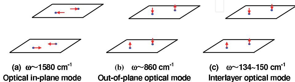
Fig. 6. Modality of atomic movements for three kinds of optical phonon modes in multilayered graphene systems.
