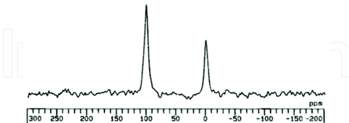
Fig. 10. Solid state ^{15}\text{N} NMR spectra of chitosan (reproduced from Yu et al., 1999).
