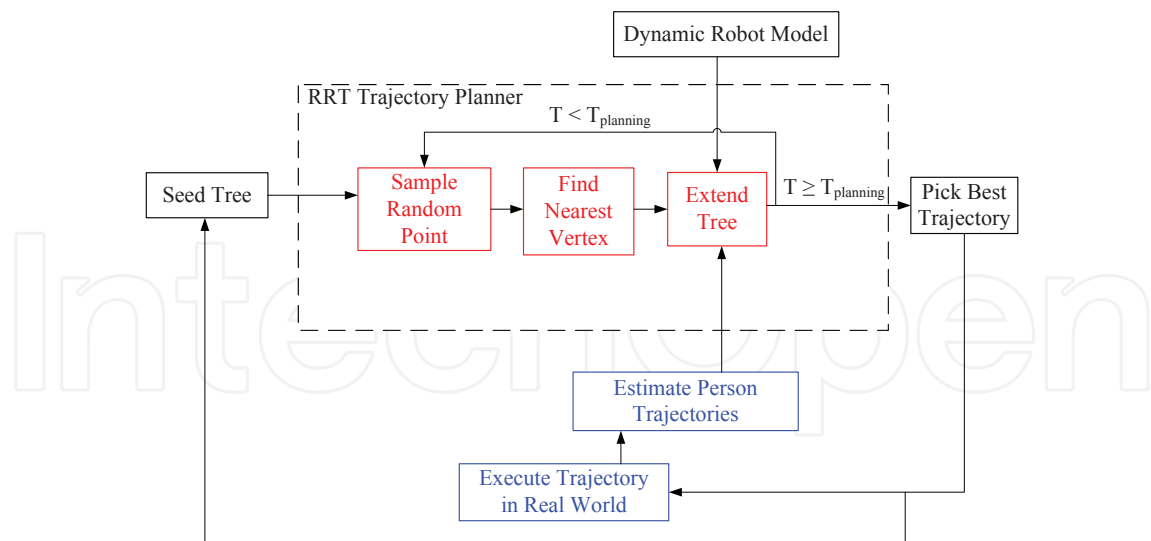
Fig. 6. The overall structure of the trajectory generator. The blue real world part and the red trajectory planning part are executed simultaneously.
