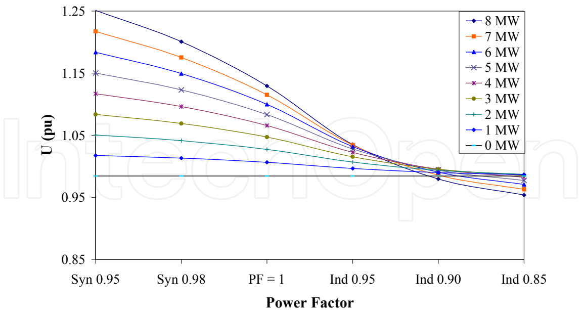
Fig. 8.5. Voltage at Node 406 with Different Power Generation Levels
