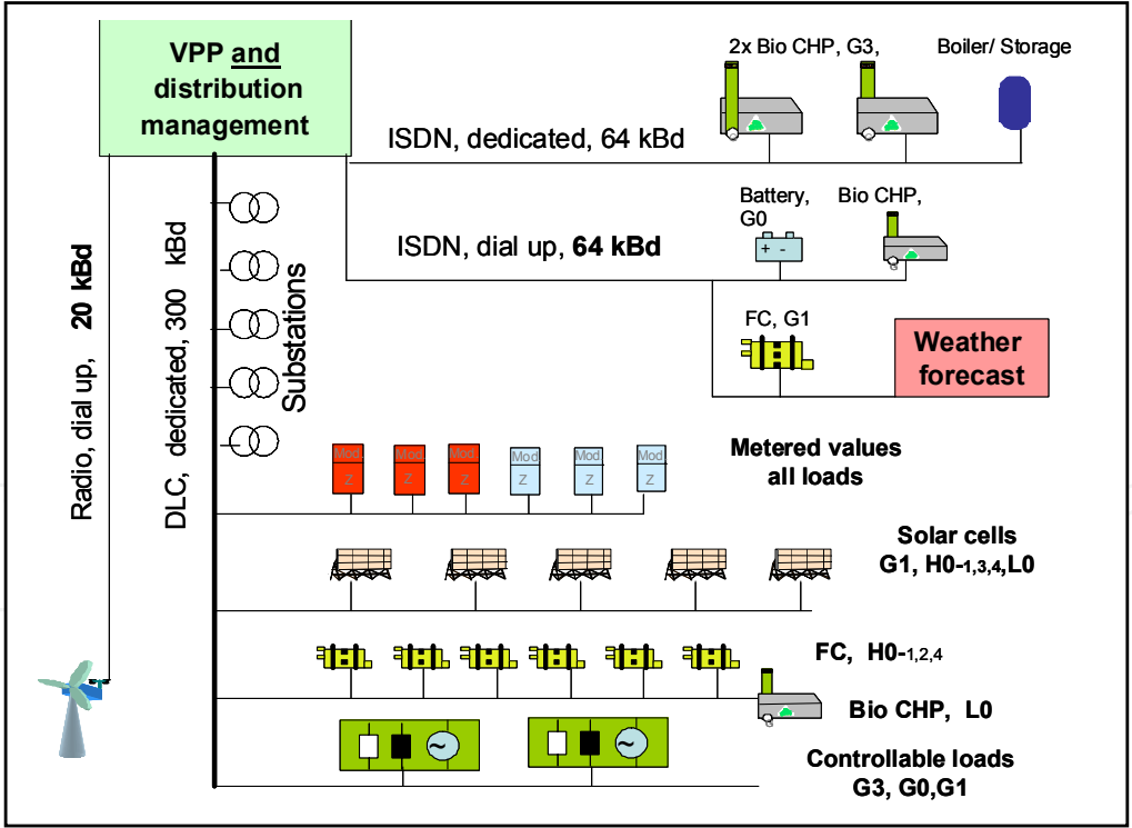
Fig. 8.15. Scheme of the Communication Network
