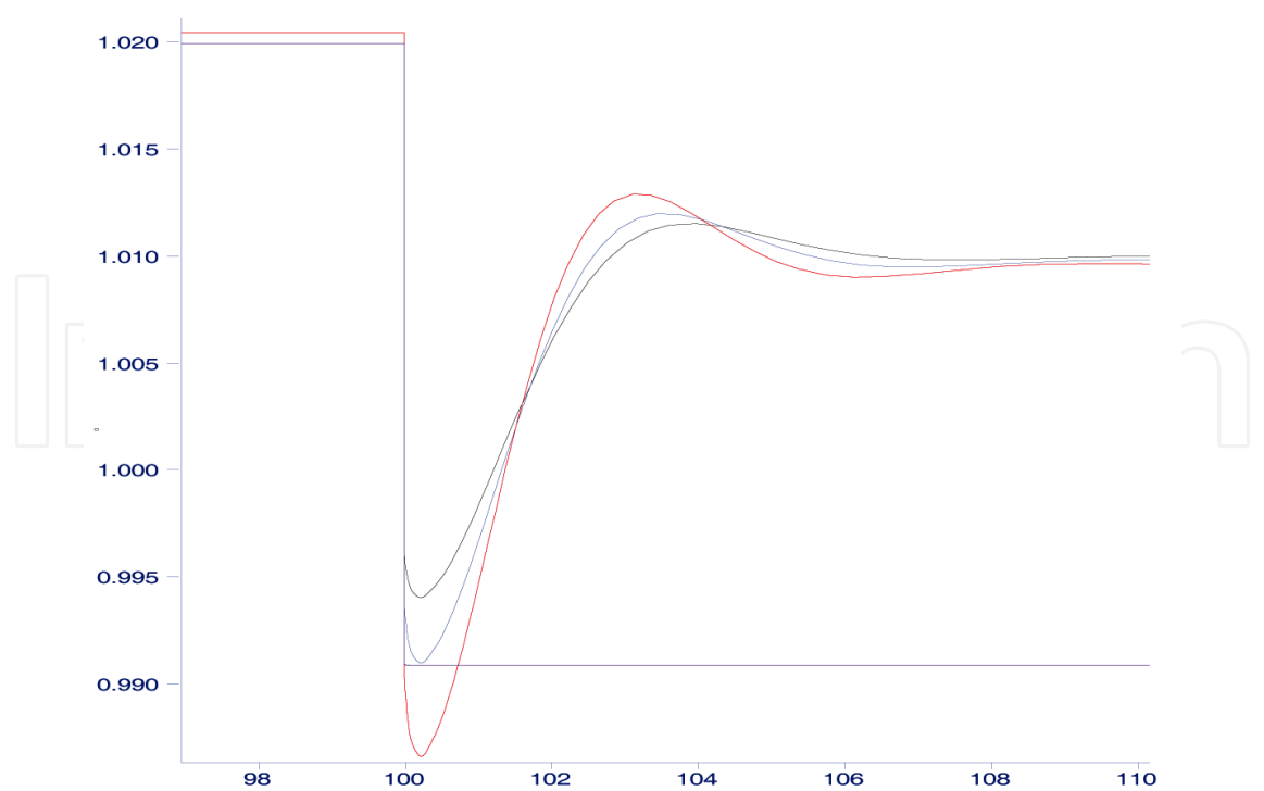
Fig. 8.7. Voltage Dip at Bus 2 with Synchronous Generator
