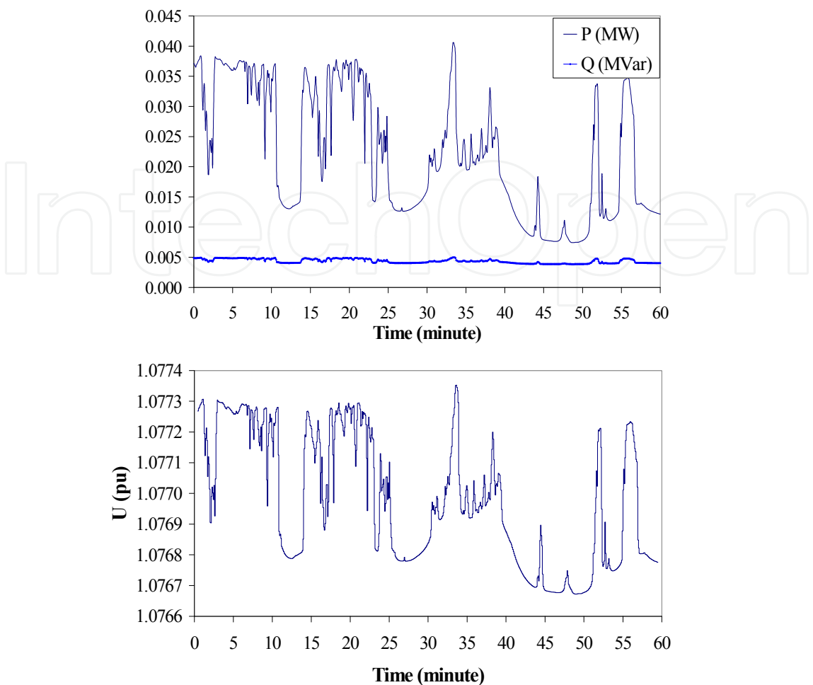
Fig. 8.6. Injected Power and Voltage at Node 304
