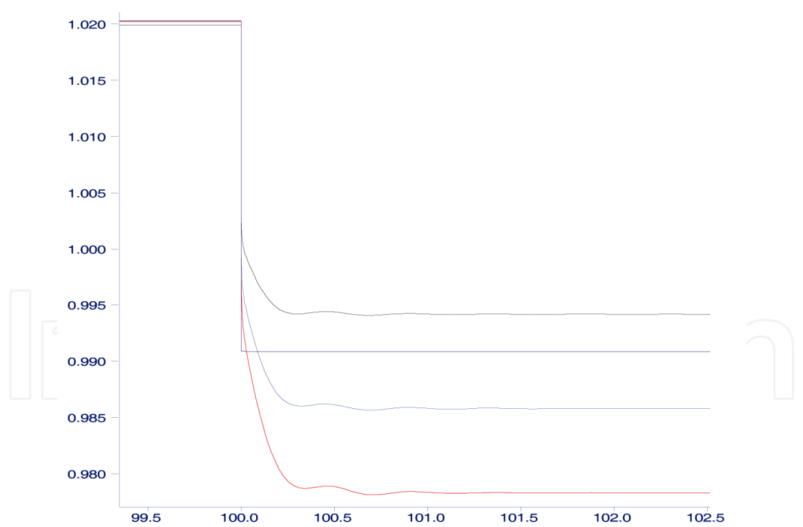
Fig. 8.8. Voltage Dip at Bus 2 with Induction Generator
