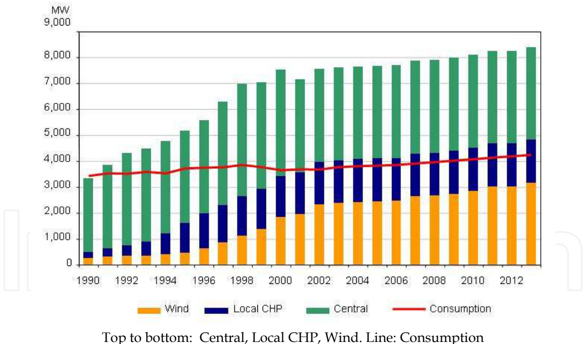
Fig. 8.18. Development of the Power Balance in Western Denmark
