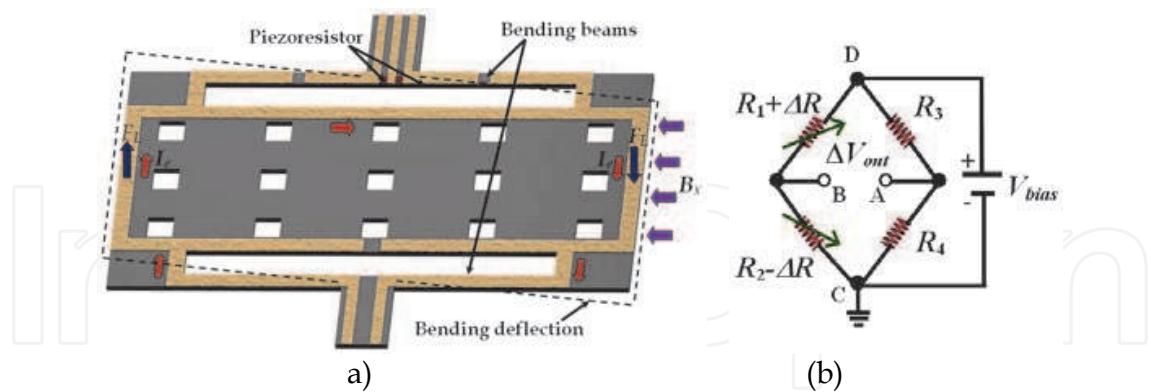
Fig. 2. A schematic view of the (a) operation principle of a resonant magnetic field microsensor with piezoresistive detection and (b) its associated Wheatstone bridge. For the two piezoresistors under a longitudinal strain ( \varepsilon_l ), their \Delta R_i is determined by (Clark and Wise, 1979)
