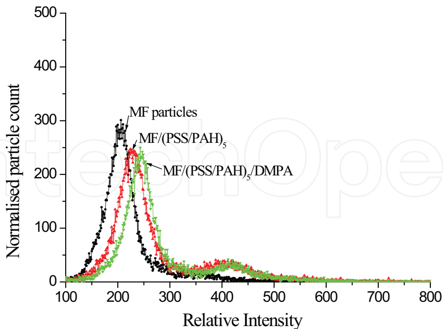
Fig. 6. Normalized light scattering intensity distributions of uncoated MF particles, MF coated with (PSS/PAH) 5 and MF/(PSS/PAH) 5 /DMPA, respectively. The diameter of MF particles used in experiment is 1.08 \pm 0.10 \mu\text{m} .
