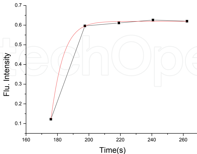
Fig. 8. Recovery profile for lipid partly coated PE capsules measured by CLSM (black dot is recorded by CLSM, red line is the fitted curve)
