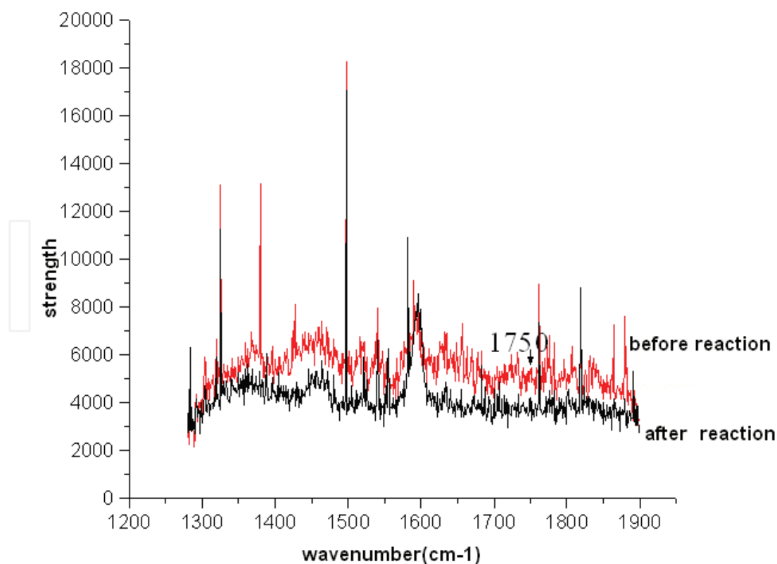
Fig. 11. Confocal laser raman spectra of capsules before and after reaction
