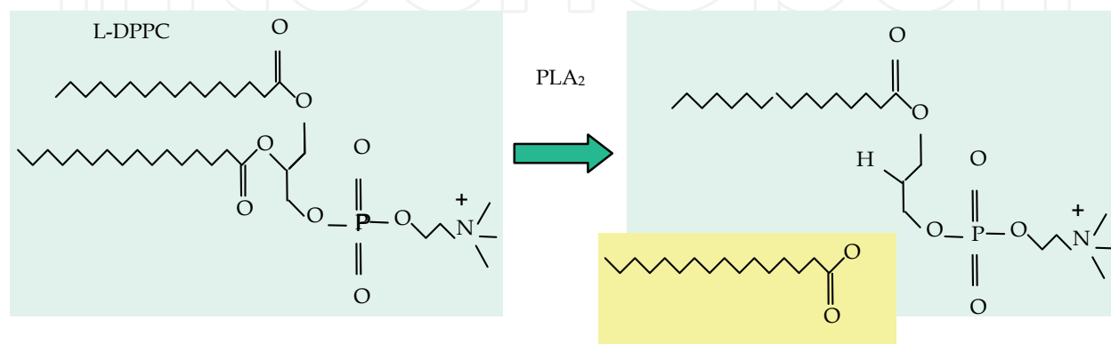
Fig. 10. Scheme for \text{PLA}_2 catalyzed L-DPPC reaction
