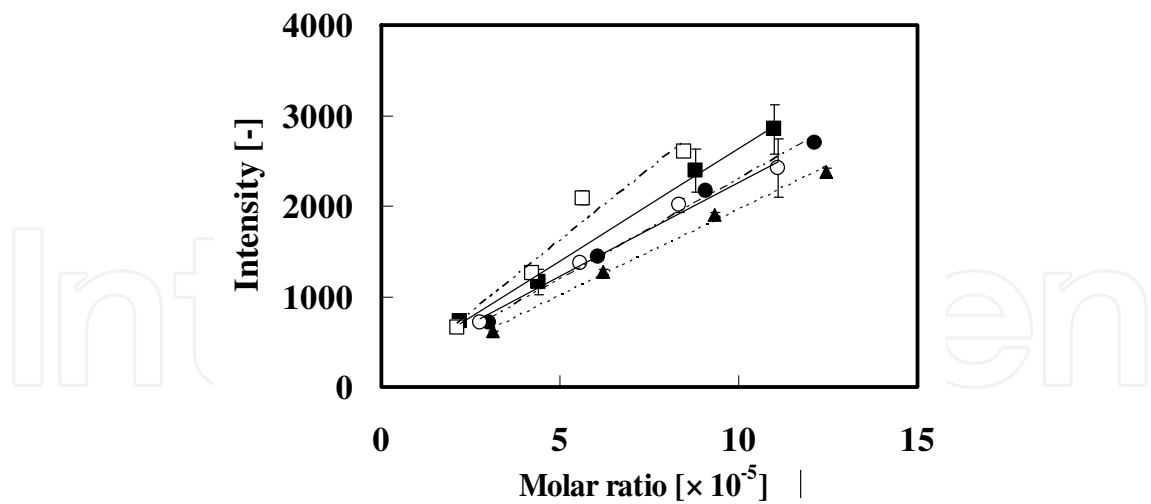
Fig. 15. Relationships between molar ratio and fluorescent intensity of perylene mixed with additives: GTA (■), TEGDA (●), BGDA (○), paraffin liquid (□) and PEG (▲).
