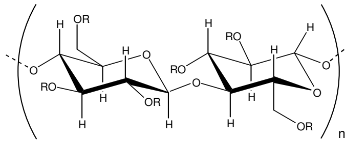
Fig. 1. Chemical structure of CA.
