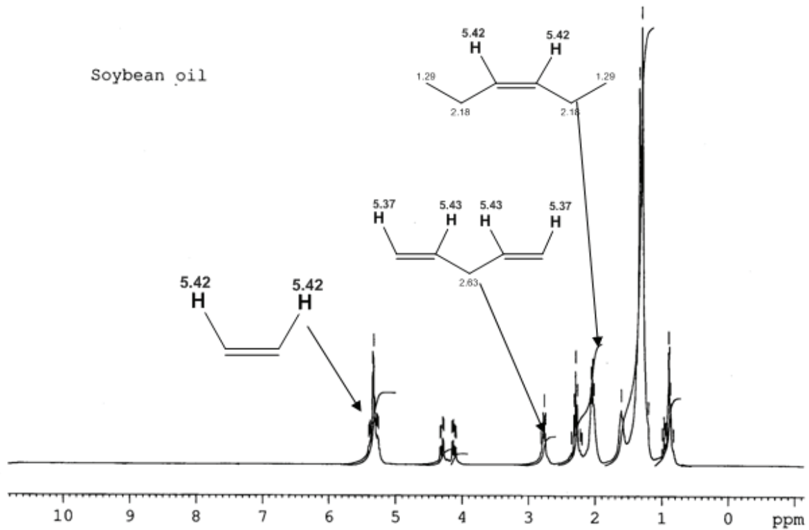
Fig. 11. 1 H NMR spectrum of initial soybean oil
