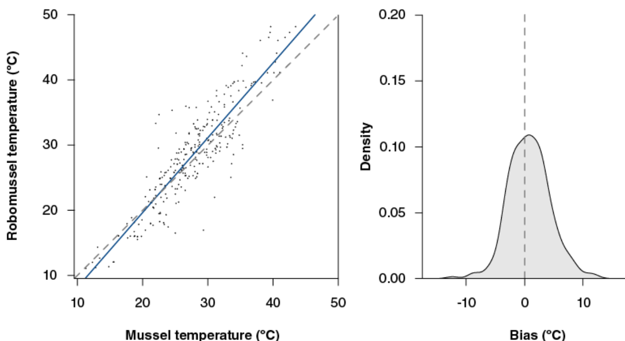
Fig. 2. Robomussel validation data (Root mean square error: 3.64^{\circ}\text{C} ). Left: correlation between mussel body temperatures and robomussel measurements in a simulated mussel bed in the lab (276 pairs of measurements from 38 independent runs). The linear correlation ( R=0.89 ) is shown in blue and the reference dashed line y=x is depicted in gray. Right: Density plot of the differences (bias) between each robomussel measurement and the correspondent body temperature (mean bias: 0.82^{\circ}\text{C} ).
