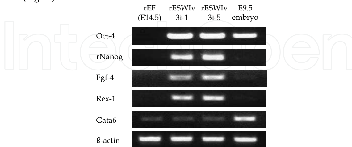
Fig. 2. Reverse transcription-PCR analysis for rat embryonic fibroblast cells at E14.5 (rEF; negative control for stem cell markers), rat embryos at E9.5 (positive control for Gata6), and two rat ES cell lines (rESWiv3i-1 and rESWiv3i-5). Both ES cell lines expressed stem cell markers, including Oct-4, rNanog, Fgf-4 and Rex-1
