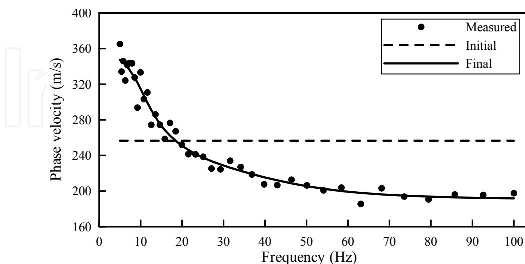
Fig. 16. Simulation results from Model D. Solid dots, dashed line, and solid line represent contaminated, initial, and calculated fundamental-mode surface wave phase velocities, respectively.
