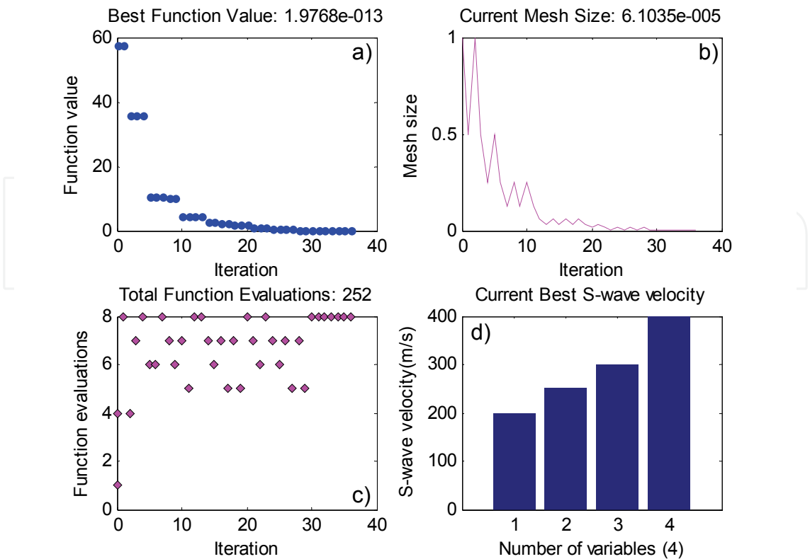
Fig. 8. Inversion results of Model D using GPS Positive Basis 2N. (a), (b), (c), and (d) have the same meaning as in Fig. 2.
