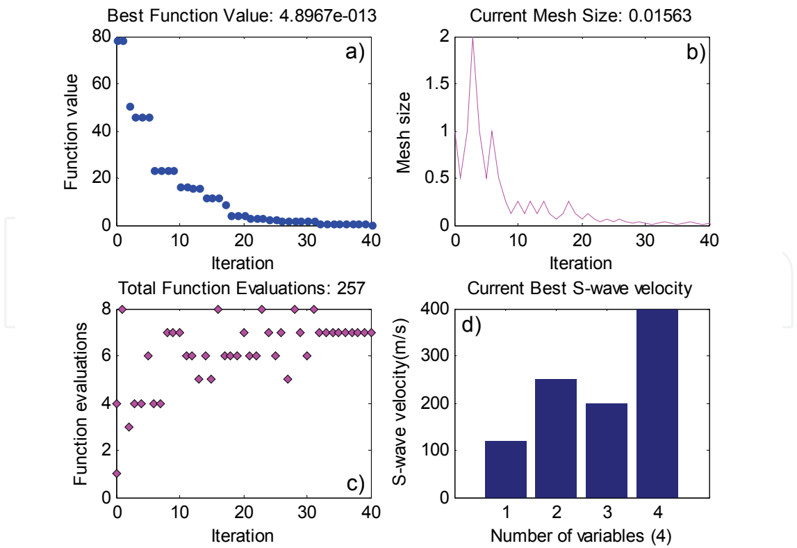
Fig. 12. Inversion results of Model F using GPS Positive Basis 2N. (a), (b), (c), and (d) have the same meaning as in Fig. 2.
