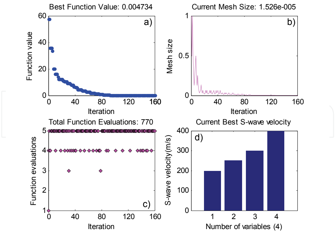
Fig. 9. Inversion results of Model D using GPS Positive Basis N+1. (a), (b), (c), and (d) have the same meaning as in Fig. 2.
