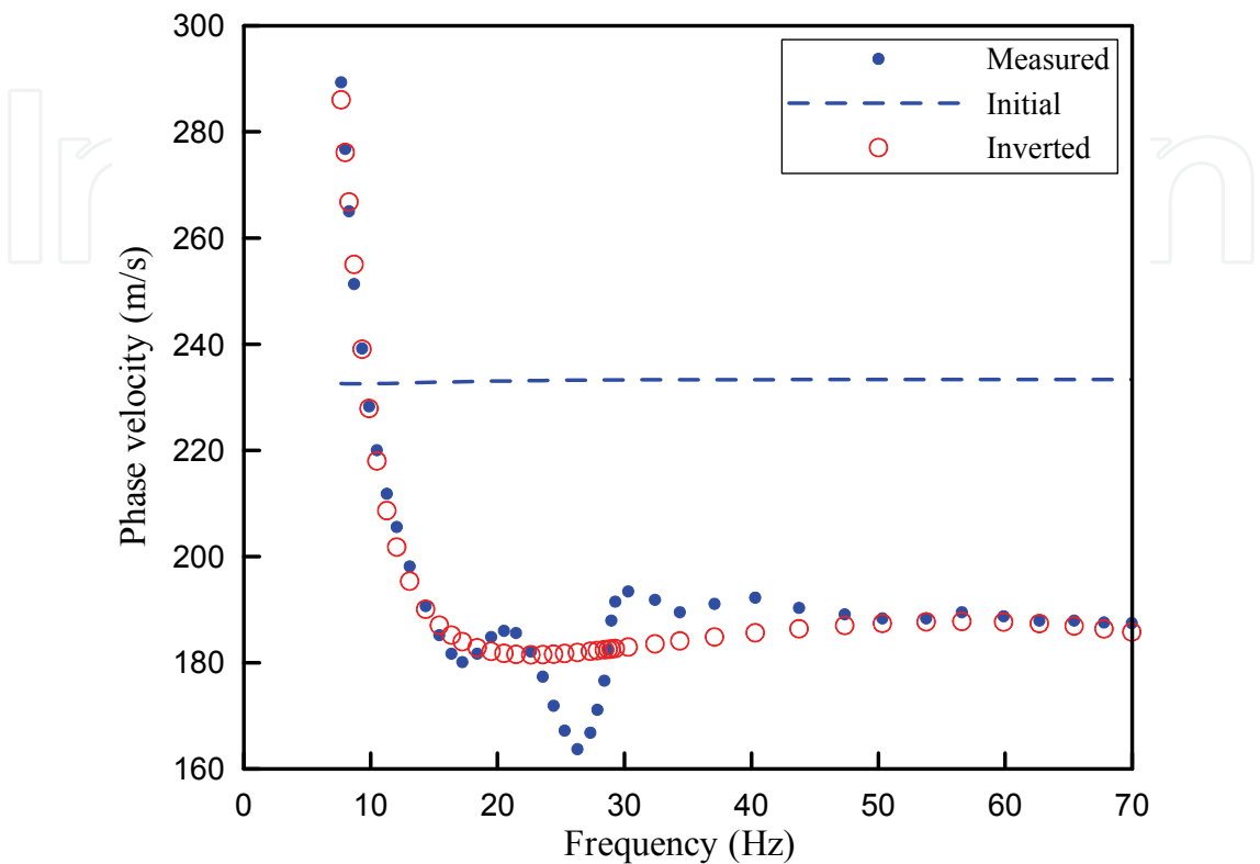
Fig. 23. A real-world example from roadbed survey in Henan, China. Solid dots, dashed line, and open circles represent measured, initial, and forwardly calculated fundamental-mode dispersion curves, respectively.
