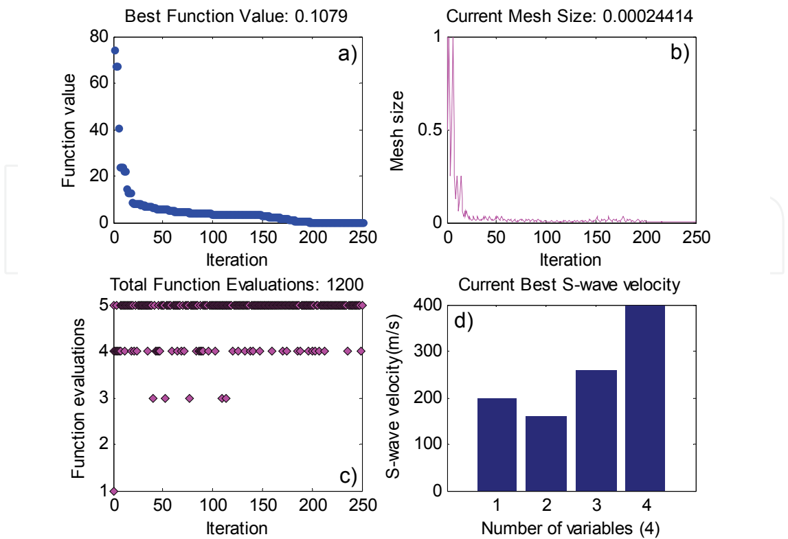
Fig. 11. Inversion results of Model E using GPS Positive Basis N+1. (a), (b), (c), and (d) have the same meaning as in Fig.2.
