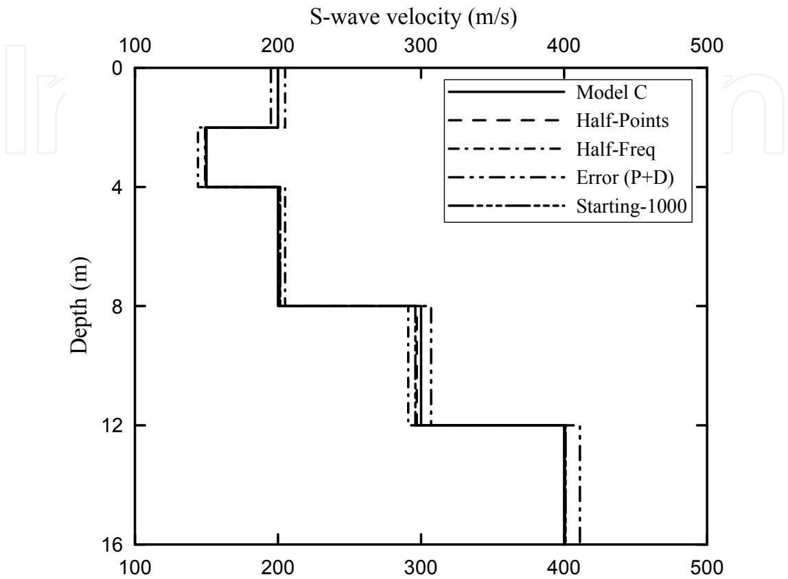
Fig. 5. Effects of the number of data points, limited frequency range, errors in P-wave velocities and density, and the starting point on inversion results of Model C using pattern search algorithms.
