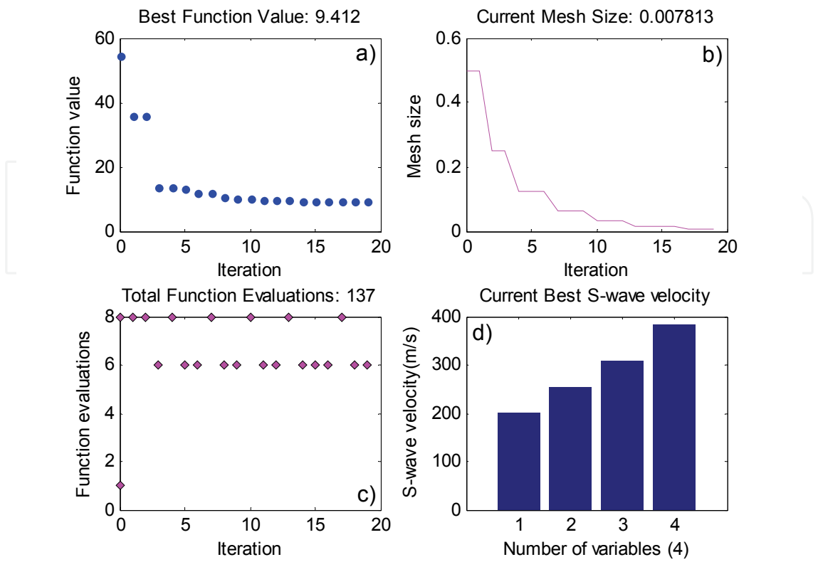
Fig. 17. Effects of inclusion of noise in surface wave data from Model D on performance of pattern search algorithm. (a), (b), (c), and (d) have the same meaning as in Fig. 2.
