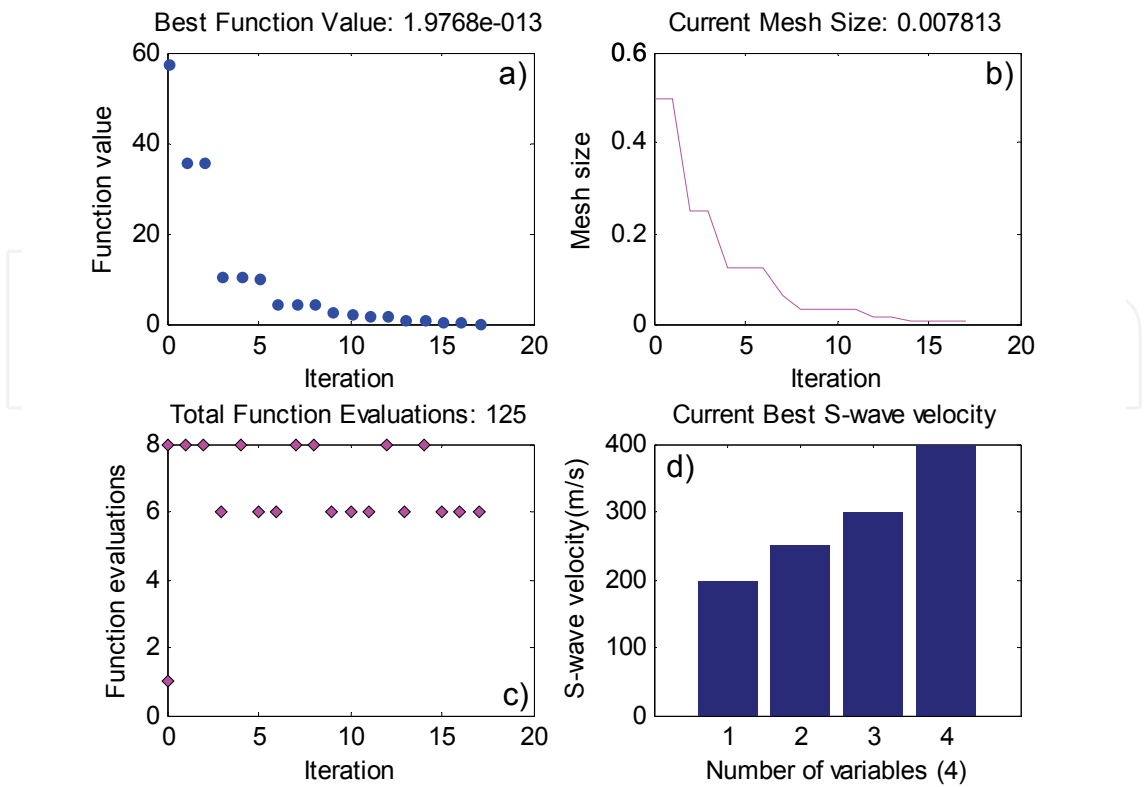
Fig. 14. Effects of expansion factor on performance of pattern search algorithm. (a), (b), (c), and (d) have the same meaning as in Fig. 2.
