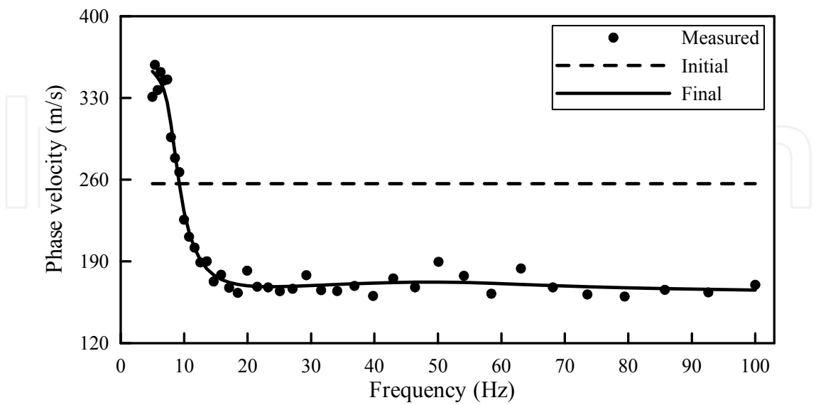
Fig. 18. Simulation results from Model E. Solid dots, dashed line, and solid line represent contaminated, initial, and calculated fundamental-mode surface wave phase velocities, respectively.
