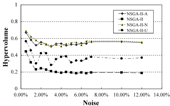
Fig. 6. Hypervolume (ch130, Normal Distribution Noise)
