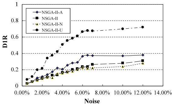
Fig. 12. D1_R (ch130, Normal Dist. Noise)
