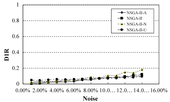
Fig. 13. D1_R (ch130, Uniform Dist. Noise)
