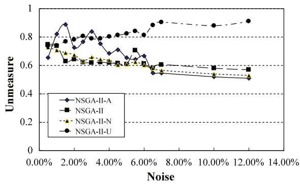
Fig. 18. U-metric (ch130, Normal Dist. Noise)
