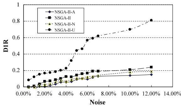
Fig. 16. D1_R (lin318, Normal Dist. Noise)
