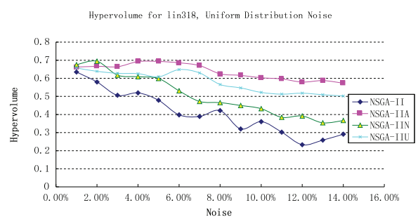
Fig. 11. Hypervolume (lin318, Uniform Distribution Noise)
