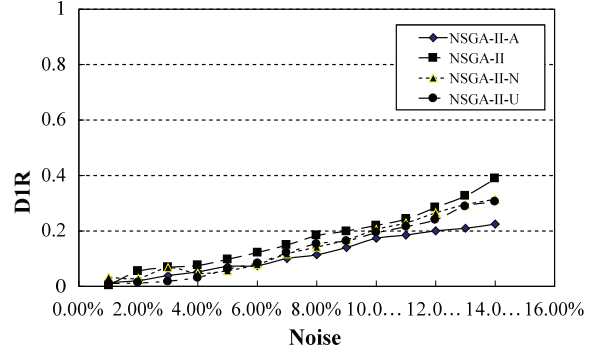
Fig. 17. D1_R (lin318, Uniform Dist. Noise)
