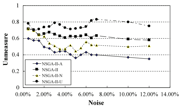
Fig. 22. U-metric (lin318, Normal Dist. Noise)
