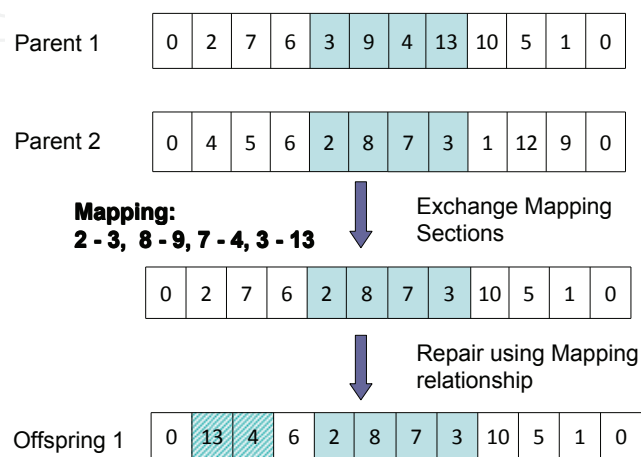
Fig. 2. An Example Crossover (PMX) Process
