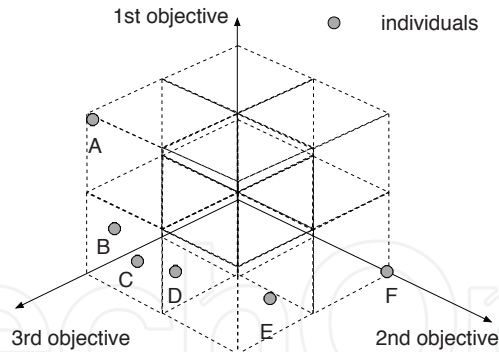
Fig. 5. An Example Hypercube in the Objective Space
