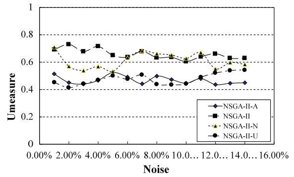
Fig. 19. U-metric (ch130, Uniform Dist. Noise)
