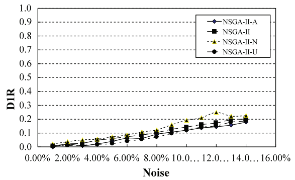
Fig. 15. D1_R (pr226, Uniform Dist. Noise)
