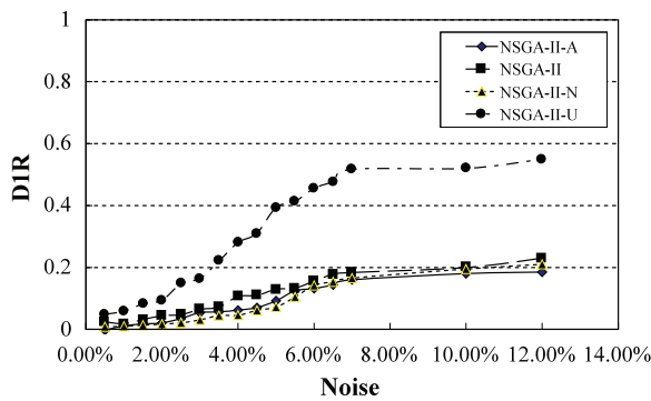
Fig. 14. D1_R (pr226, Normal Dist. Noise)
