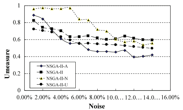
Fig. 21. U-metric (pr226, Uniform Dist. Noise)
