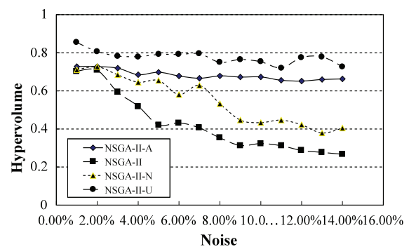
Fig. 7. Hypervolume (ch130, Uniform Distribution Noise)
