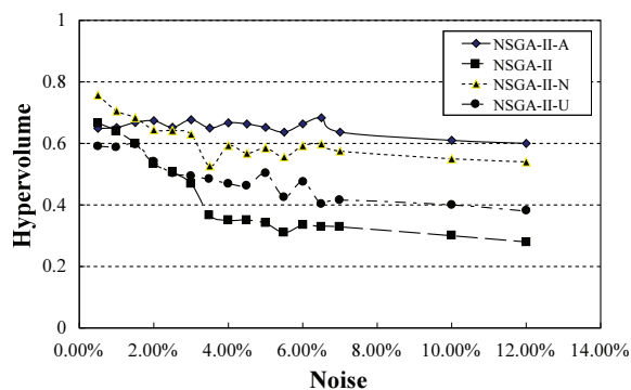
Fig. 10. Hypervolume (lin318, Normal Distribution Noise)
