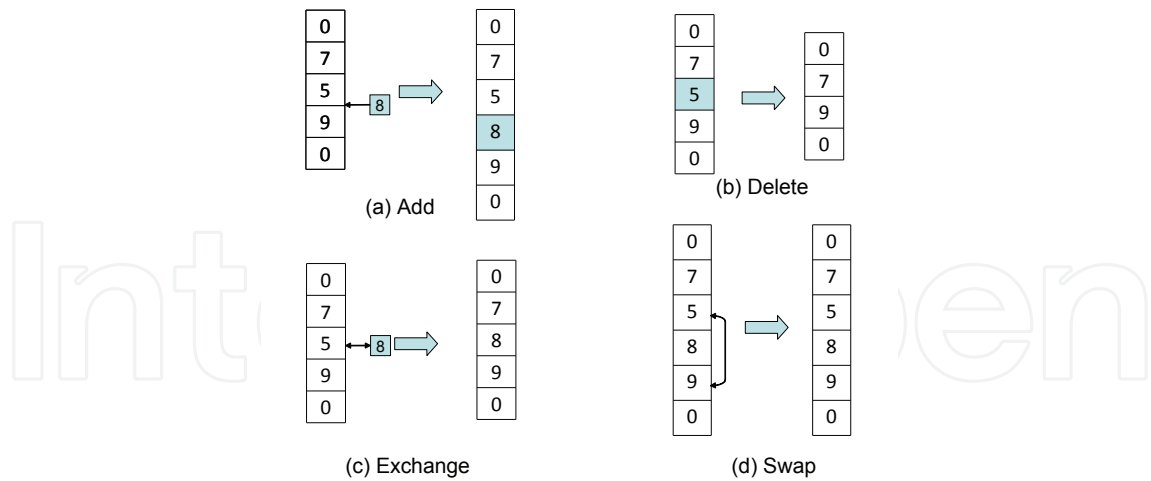
Fig. 3. Example Mutation Processes
