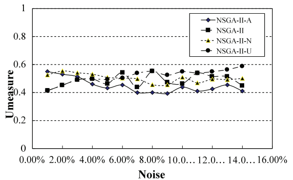
Fig. 23. U-metric (lin318, Uniform Dist. Noise)
