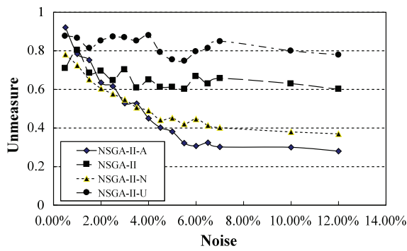
Fig. 20. U-metric (pr226, Normal Dist. Noise)
