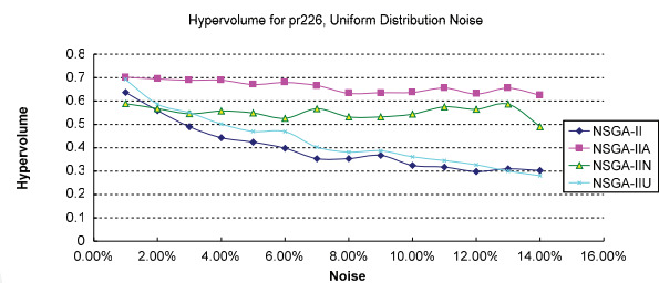
Fig. 9. Hypervolume (pr226, Uniform Distribution Noise)
