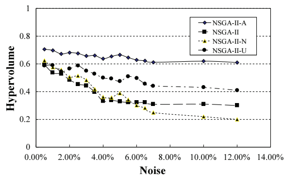
Fig. 8. Hypervolume (pr226, Normal Distribution Noise)
