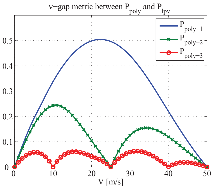
(b) polytopic models
