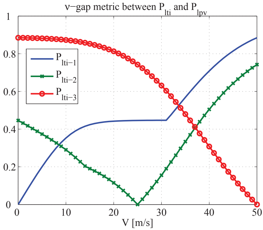
(a) LTI models
