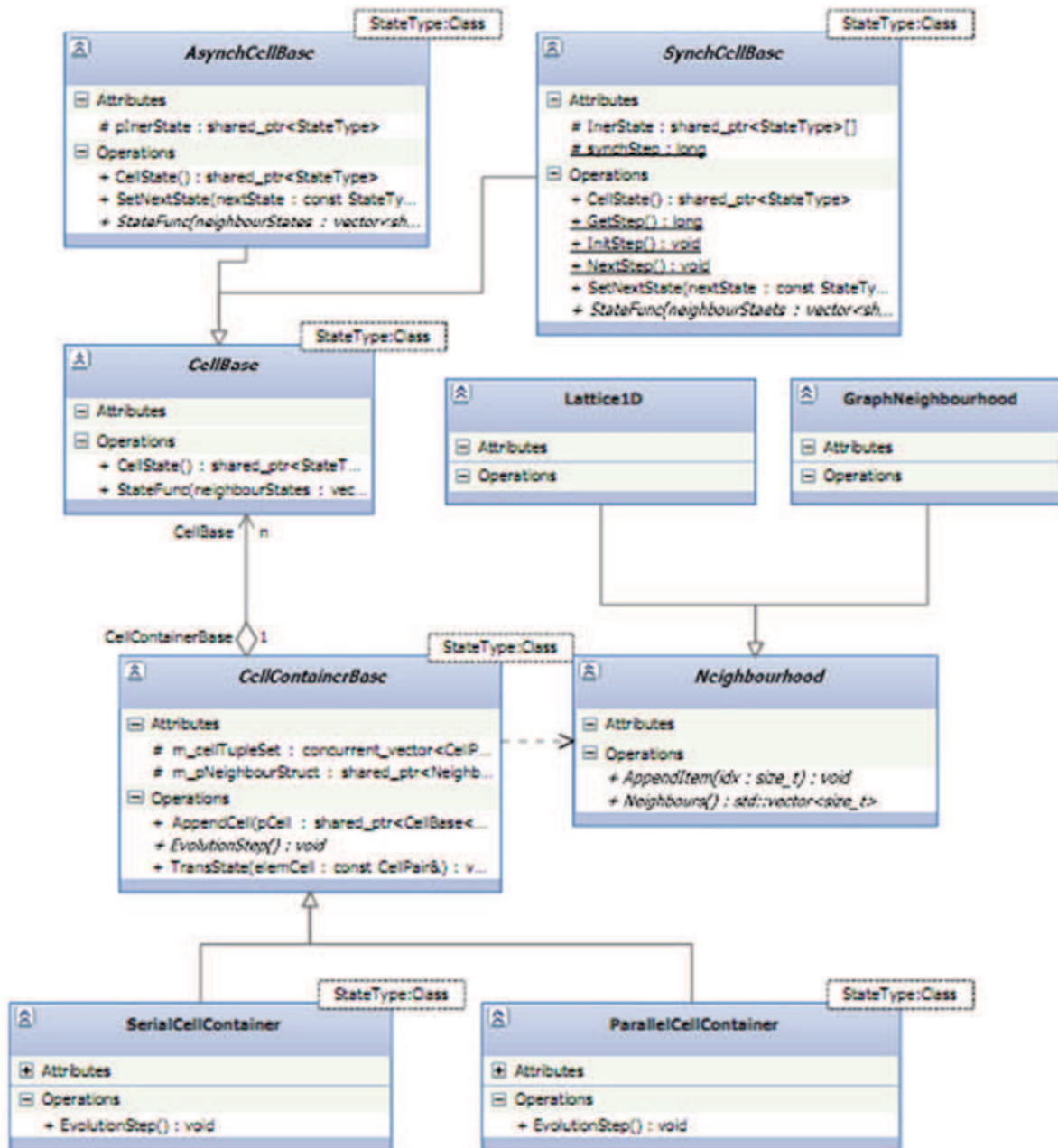
Fig. 2. Static Structure of Cellular Automata Library
