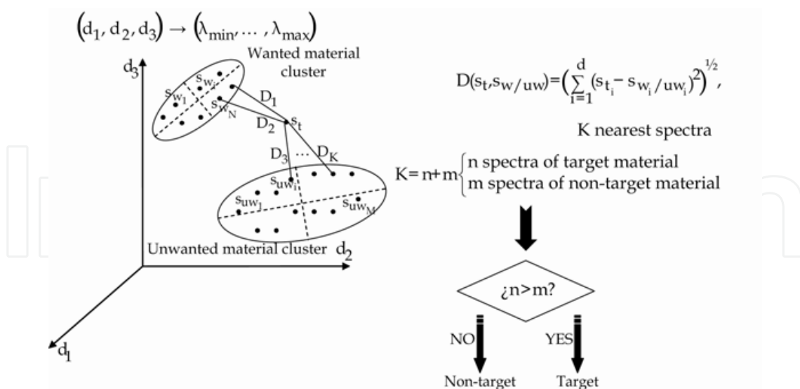
Fig. 11. KNN classifier where each feature is considered as a coordinate axis and the distance between points in this space determines how similar or different they are
