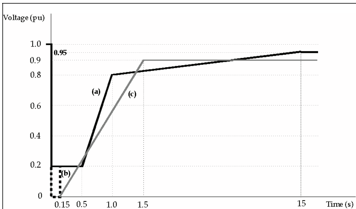
Fig. 2. Low Voltage Ride Through requirements: (a) Spanish O.P. 12.3, (b) Spanish O.P. 12.2 (draft), (c) E.ON Netz
