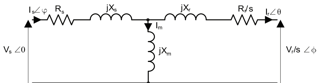
Fig. 3. DFIG Equivalent circuit.
