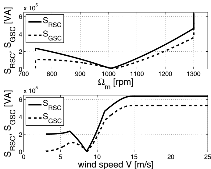
Fig. 12. RSC and GSC apparent power for GPF=1.
