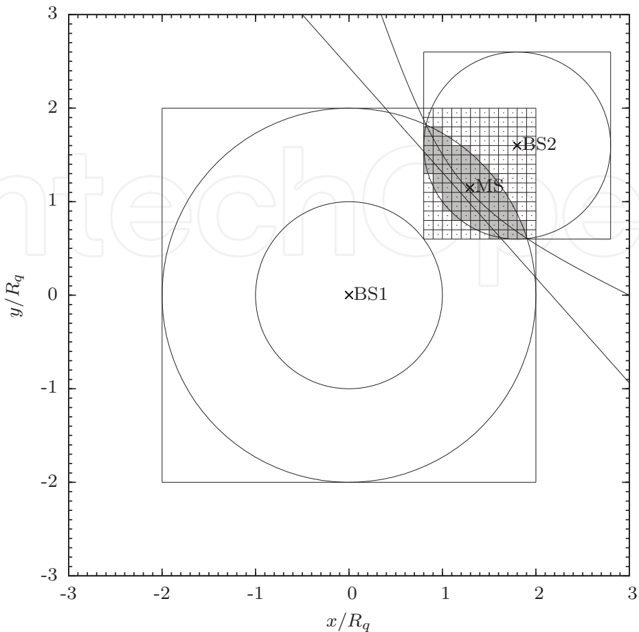
Fig. 6. Probabilistic methods, an example.
