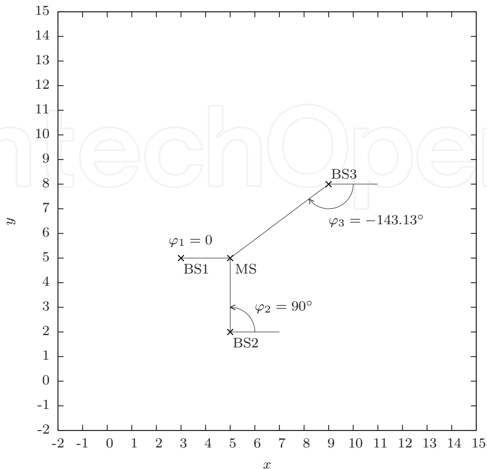
Fig. 2. Angulation.
