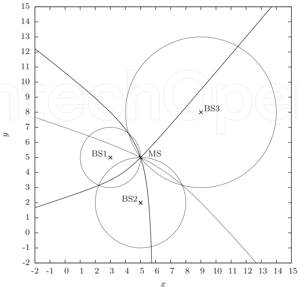
Fig. 4. Hyperbolic lateration, unique solution.
