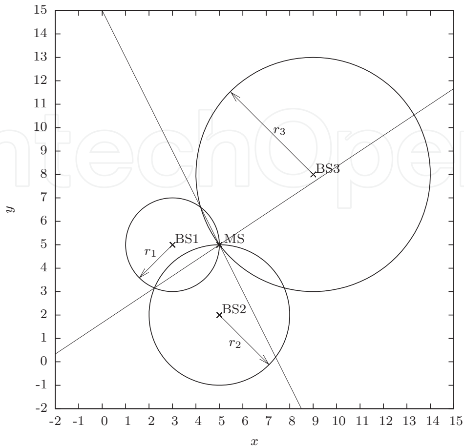
Fig. 3. Circular trilateration.
