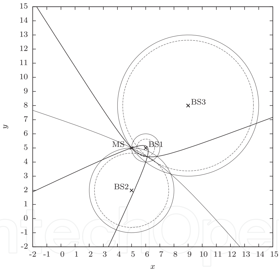
Fig. 5. Hyperbolic lateration, pair of solutions.
