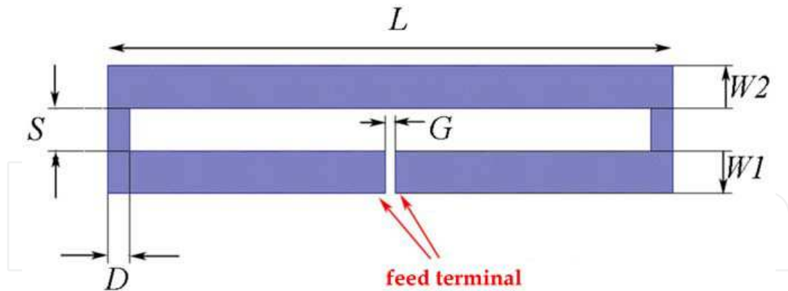
Fig. 6. Dimensions and parameters of the coplanar strip folded dipole.
