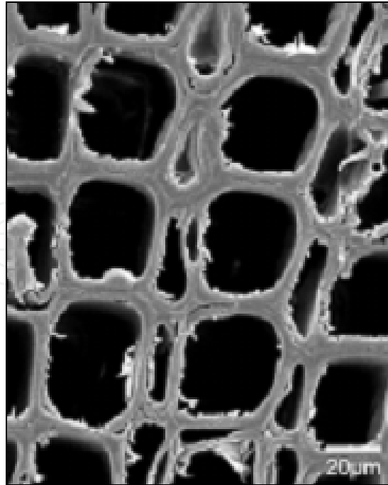
Fig. 5. SEM micrographs of treated pine sapwood sample
