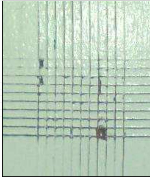
Fig. 13. Cross-cut testing carried out on aqueous based coating applied on densified composite
