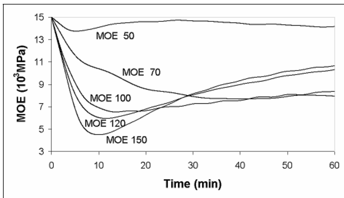
Fig. 3. Young's modulus behaviour of impregnated beech veneer samples subjected to isothermal conditions at 50, 70, 100, 120 and 150 ^{\circ}\text{C}
