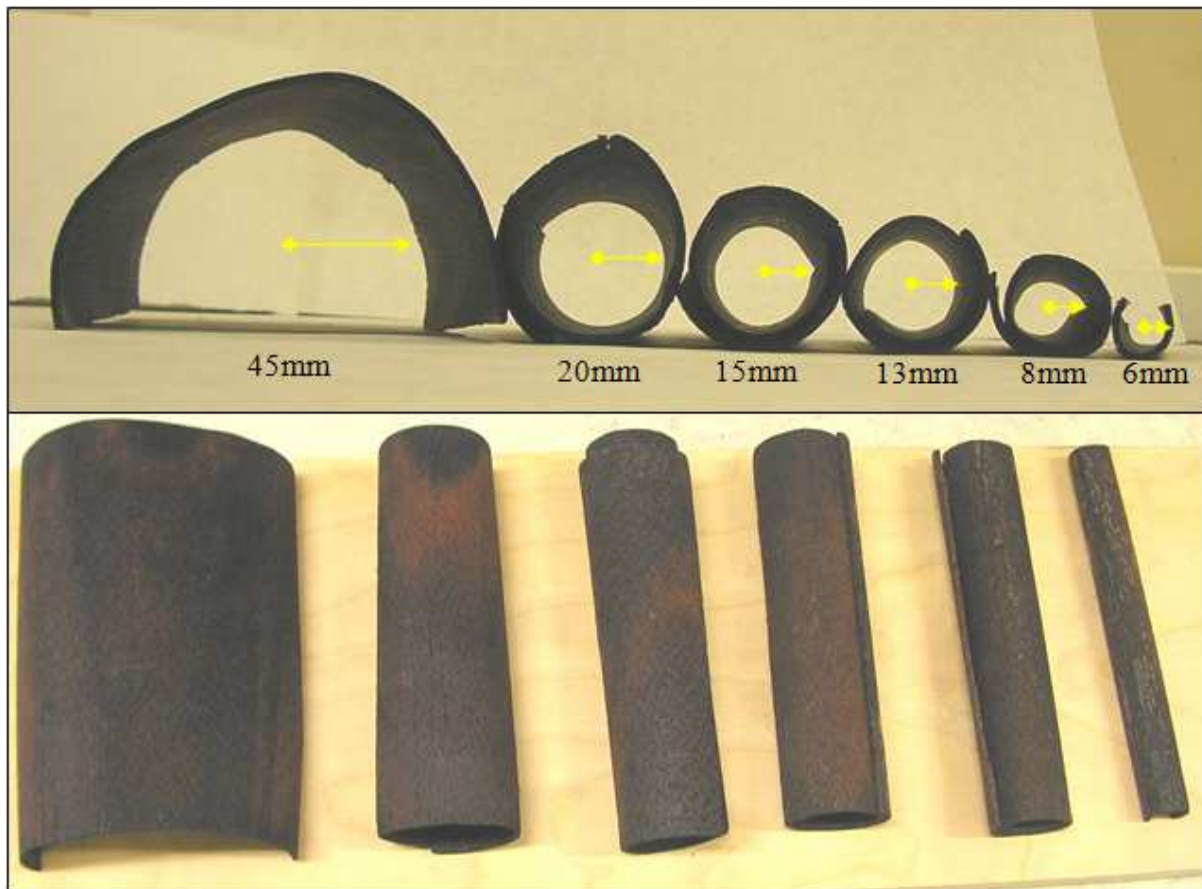
Fig. 12. Moulded and fixed samples
