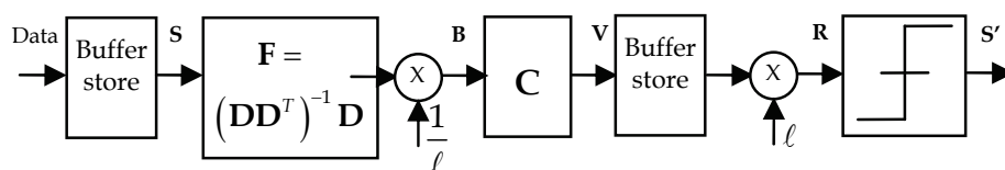
Fig. 7. Final block diagram of the precoding system
