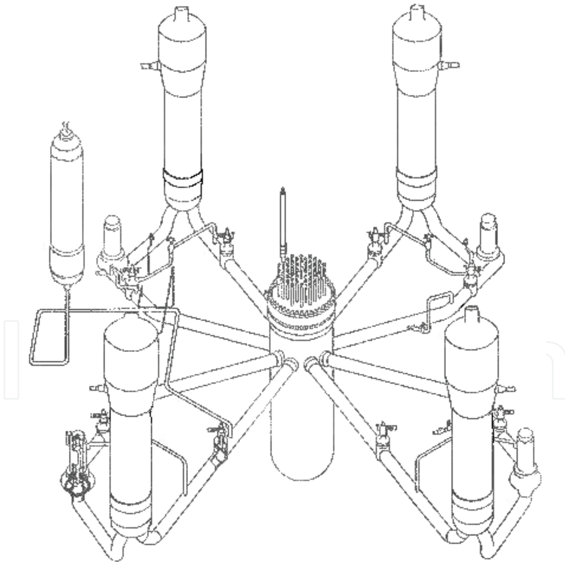
Fig. 2. General scheme of PWR primary circuit
