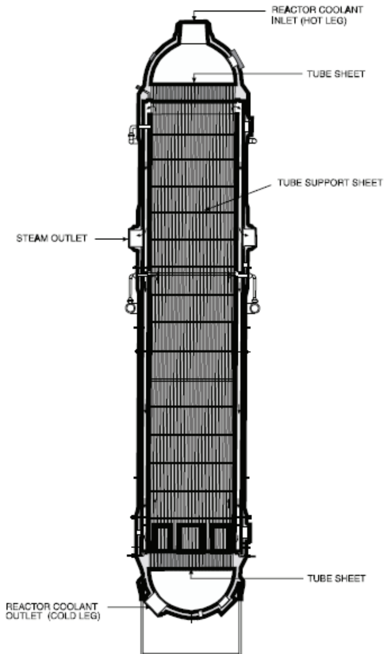
Fig. 3c. Typical Babcock & Wilcox Once through steam generator
