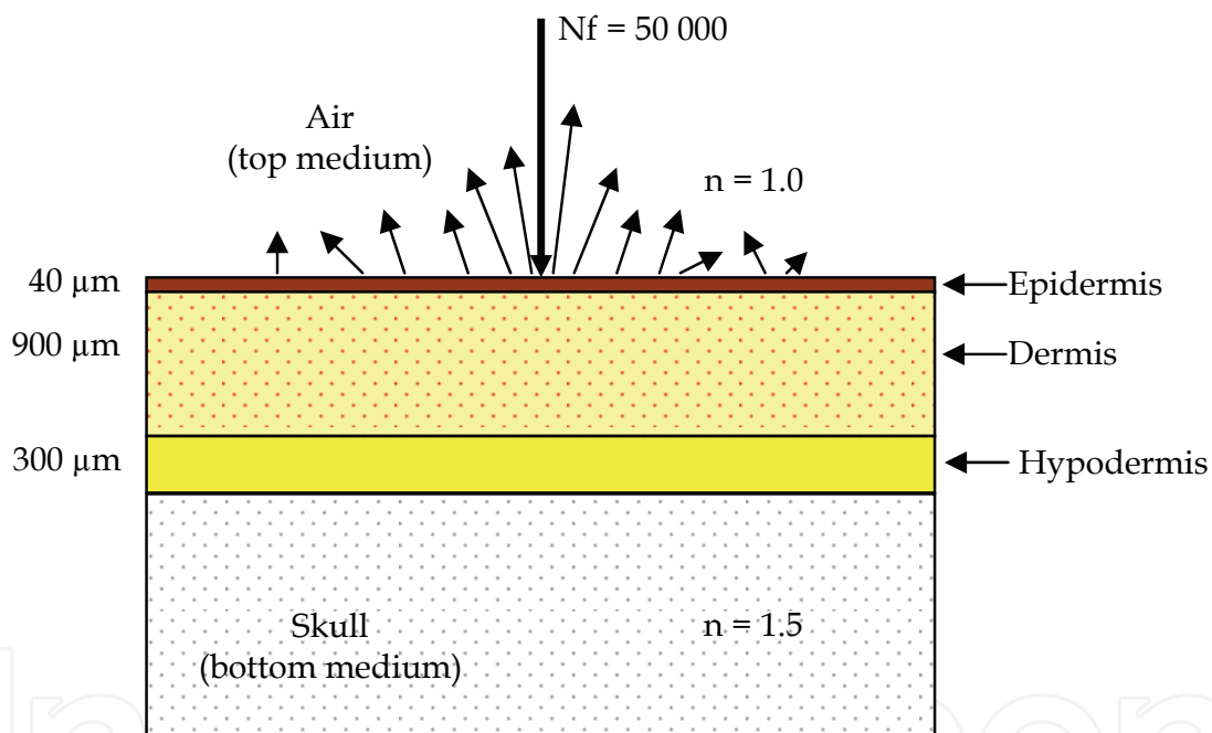
Fig. 1. Schematic representation of the three-layer skin model of the forehead of newborn infants. The skin is considered as a 3-D half-infinite medium divided into three layers: epidermis, dermis and subcutaneous tissue (or hypodermis). The top medium is the air surrounding epidermis and the bottom medium is the skull.
