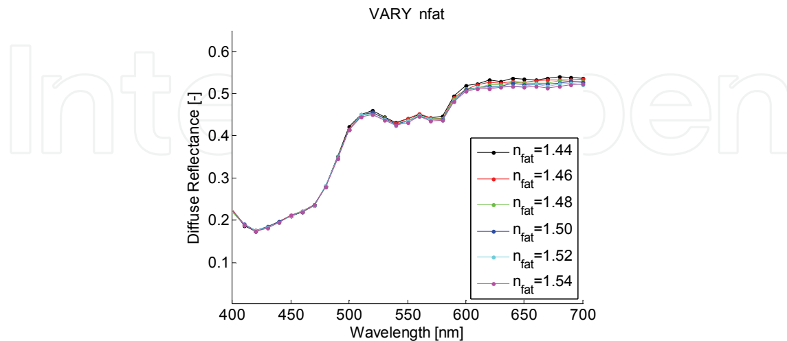
Fig. 6. Diffuse reflectance spectra of neonatal skin for various refractive index of subcutaneous tissue while the remaining parameters ( C_{bi} = 0.1 g/L, f_{bl} = 0.002 , f_{me} = 0.02 and n_{skull} = 1.50 ) of the model are kept constant.
