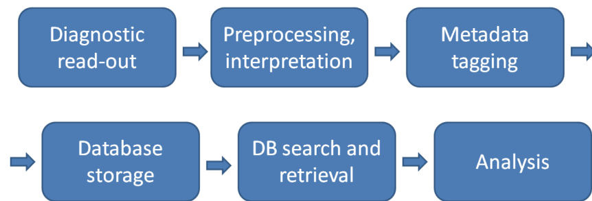
Fig. 3. Typical information flow in automotive diagnostics
