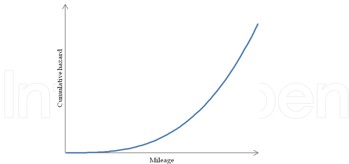
Fig. 6. Cumulative hazard function
