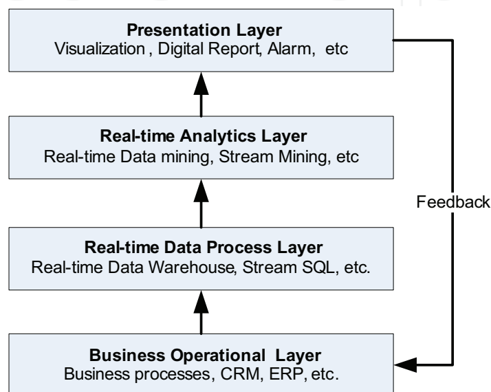
Fig. 1. Four-layer Framework
