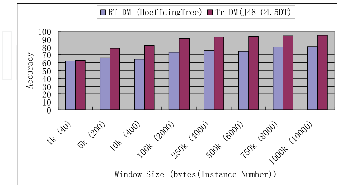
Fig. 9. Average Predication Accuracy Comparison by Window Sizes
