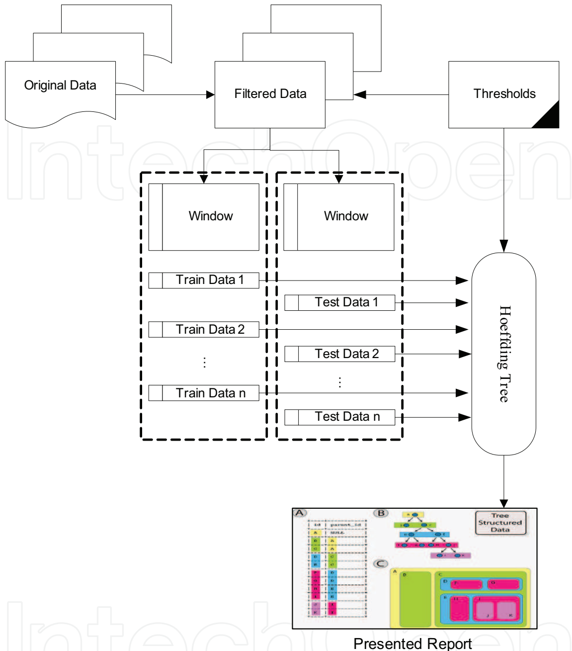
Fig. 4. Procedure Workflow
