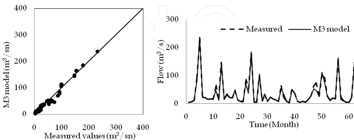
Fig. 2. Comparison of flow values of measured and the M3 model developed multilinear regression algorithm
