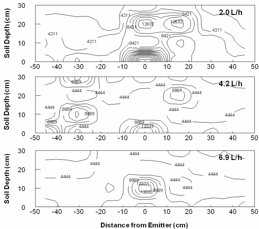
Fig. 12. Contour of EPF concentration in the soil within the 30 cm by 91.2 cm cross section area under the emitters at flow rates of 2.0, 4.2 and 6.9 L/h, respectively.
