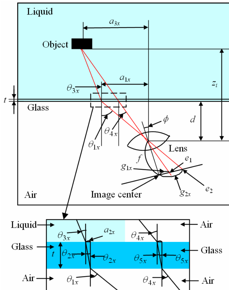
Fig. 6. Image restoration.
