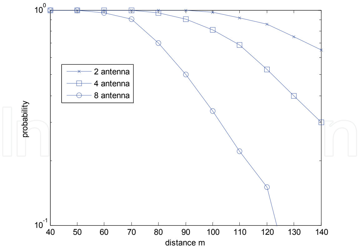
Fig. 14. Probability of correct receiving a data packet by varying the distance and number of transmitter antennas
