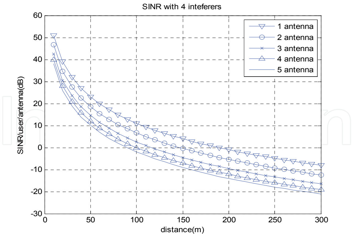
Fig. 4. SINR per user for receiving antenna by varying the distance
