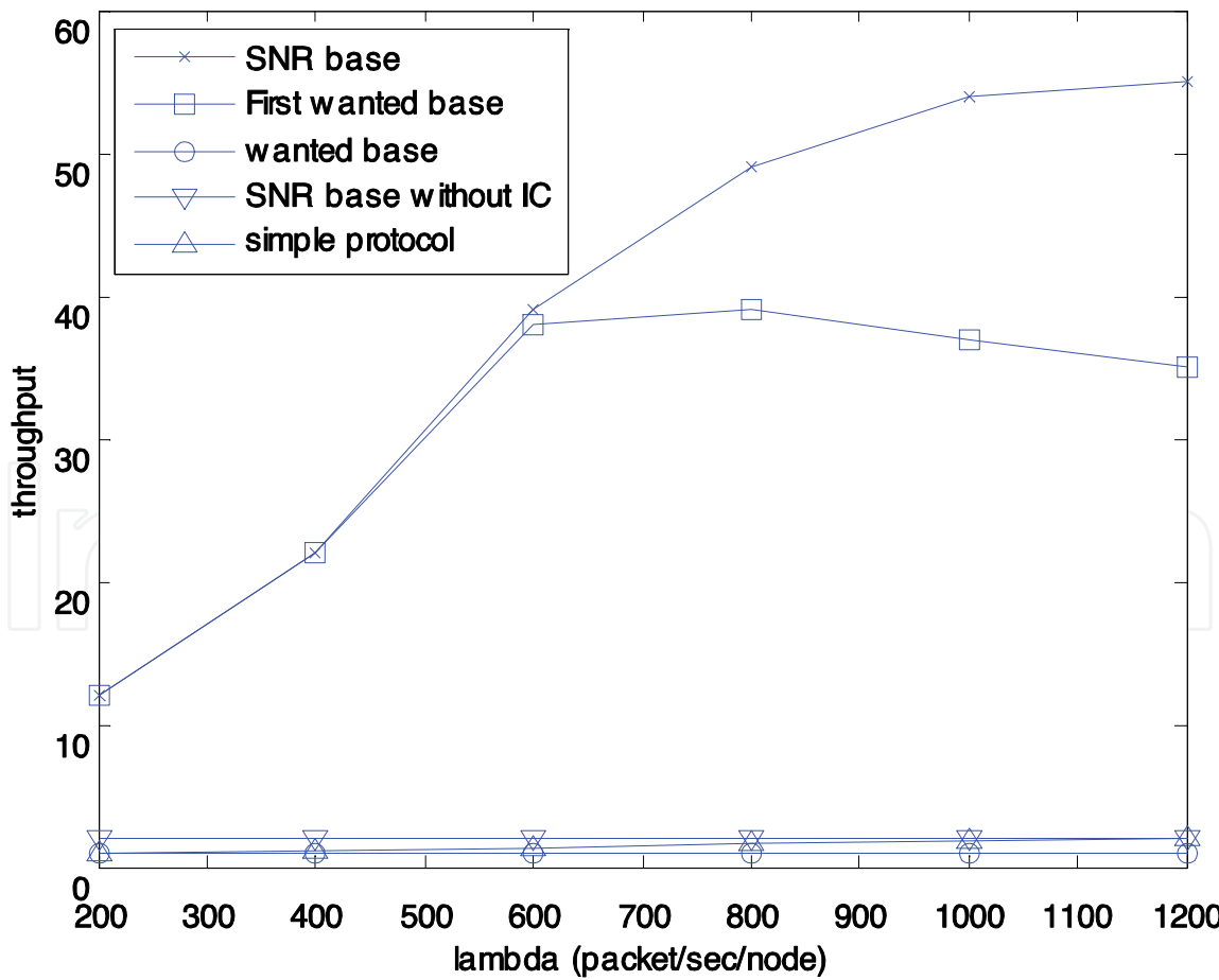
Fig. 26. Network throughput versus network traffic.
