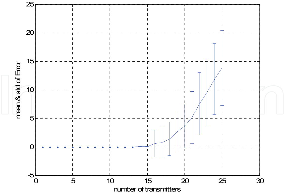
Fig. 8. Mean and standard deviation of bit errors for 1-24 RTS packets
