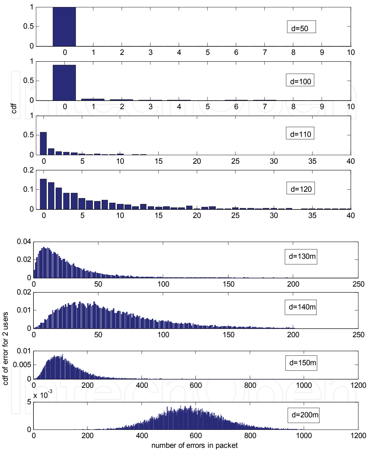
Fig. 6. Distributions of errors for data packets transmitted by 2 users each with 4 antennas by varying the distance Fig. 8. shows the average error and standard deviation of the number of errors in the RTS packets, which are sent from 1 to 24 transmitters and are placed at 100m with 8 interferers which are placed at 300m are sending packets simultaneously. The standard deviation gives an idea of the magnitude, which distributes the number of errors: the error will increase by growth in the number of packets.
