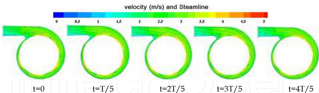
Fig. 18. Unsteady flow calculation results of absolute velocity and streamlines in volute at the large flow rate case ( Q=124\%Q_d )
