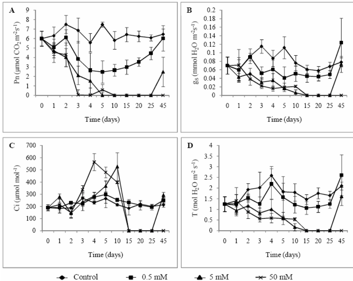
Fig. 2. Changes in net photosynthesis ( P_n ) (A), stomatal conductance ( g_s ) (B), intercellular \text{CO}_2 concentration ( C_i ) (C), and transpiration rate ( T ) (D) in leaves of grapevine after the spraying of various fmx concentrations. Each value is the mean of 15 measurements \pm SD.
