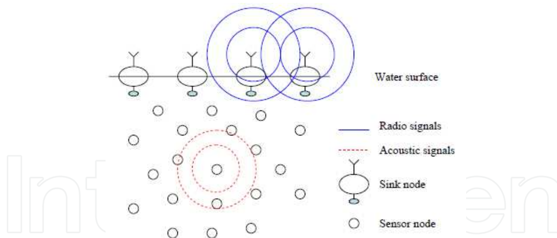
Fig. 9. Multiple sink underwater sensor network architecture
