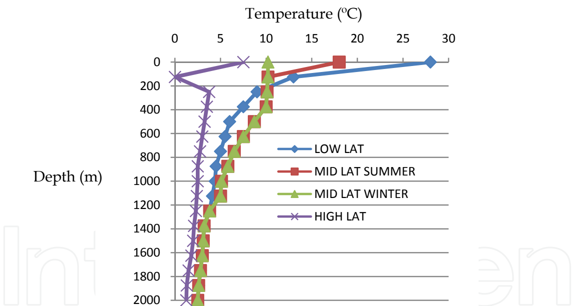
Fig. 2. Temperature variation depending on latitude and season
