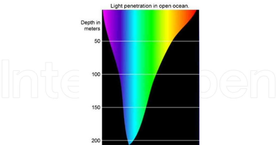
Fig. 1. This diagram offers a basic illustration of the depth at which different colors of light penetrate ocean waters. Water absorbs warm colors like reds and oranges and scatters the cooler colors
