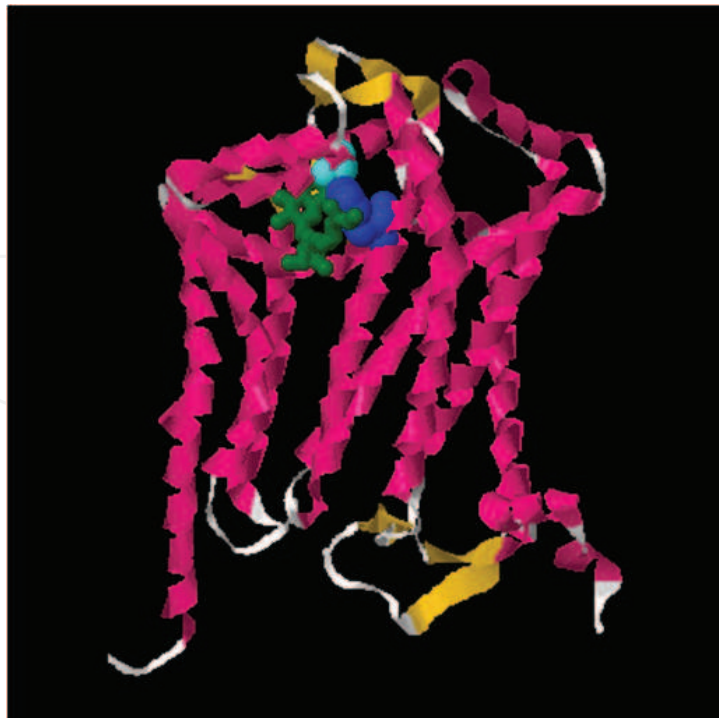
Fig. 7. Cytochrome b and QoI resistance. Molecular model of the cytochrome b protein of Saccharomyces cerevisiae . A QoI fungicide molecule bound to the Qo site of the cytochrome bc 1 complex is depicted in green. The amino acids substitutions G143A and F129L that are responsible for QoI resistance are depicted in cyan and blue, respectively. Note how these amino acids interact with the fungicide molecule.
