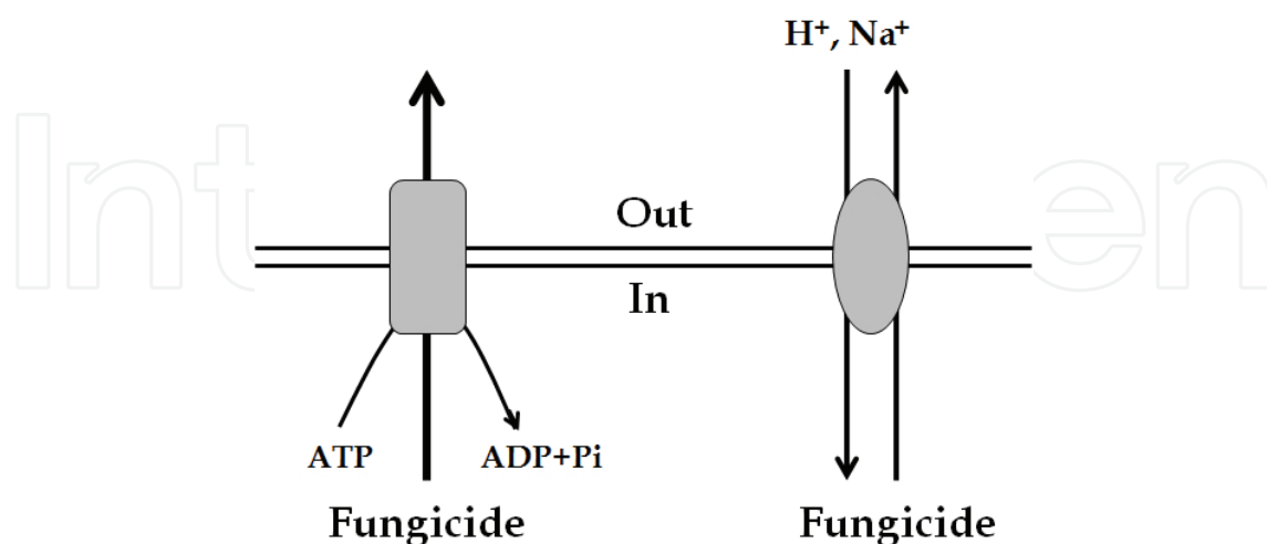
Fig. 8. Schematic representation of the two major classes of efflux transporters in fungi. ATP-binding cassette (ABC) transporters utilise the free energy of ATP hydrolysis to pump fungicides out of the cell. The transporters from the major facilitator superfamily (MFS) mediate the extrusion of fungicides in a coupled exchange with protons or sodium ions.
