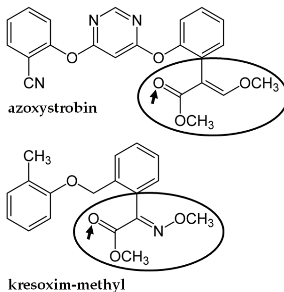
Fig. 2. The chemical structures of azoxystrobin and kresoxim-methyl. The (E)- \beta -methoxyacrylate group of azoxystrobin and the methoxyiminoacetate group of kresoxim-methyl are highlighted with circles and the carbonyl oxygen moieties responsible for binding are indicated by the arrow.
