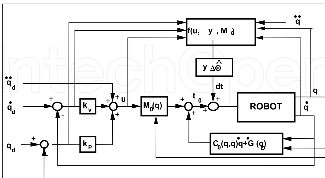
Fig. 3. Amestegui's adaptive compensation scheme
