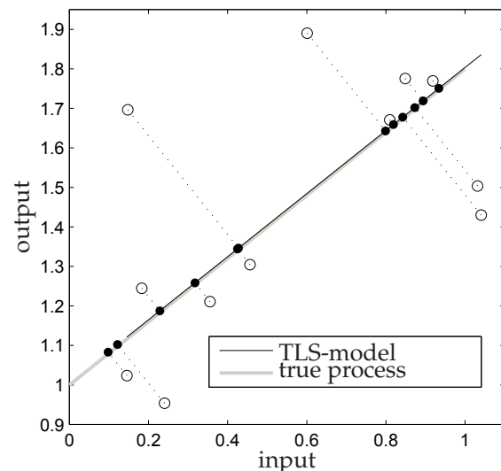
Fig. 7. Linear model, optimised by Total Least Squares
