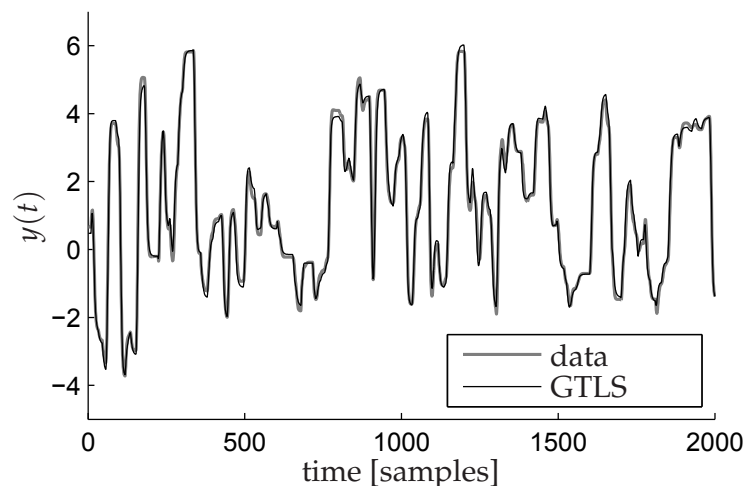
Fig. 11. Comparison of validation data to nonlinear models with GTLS parameter estimates
