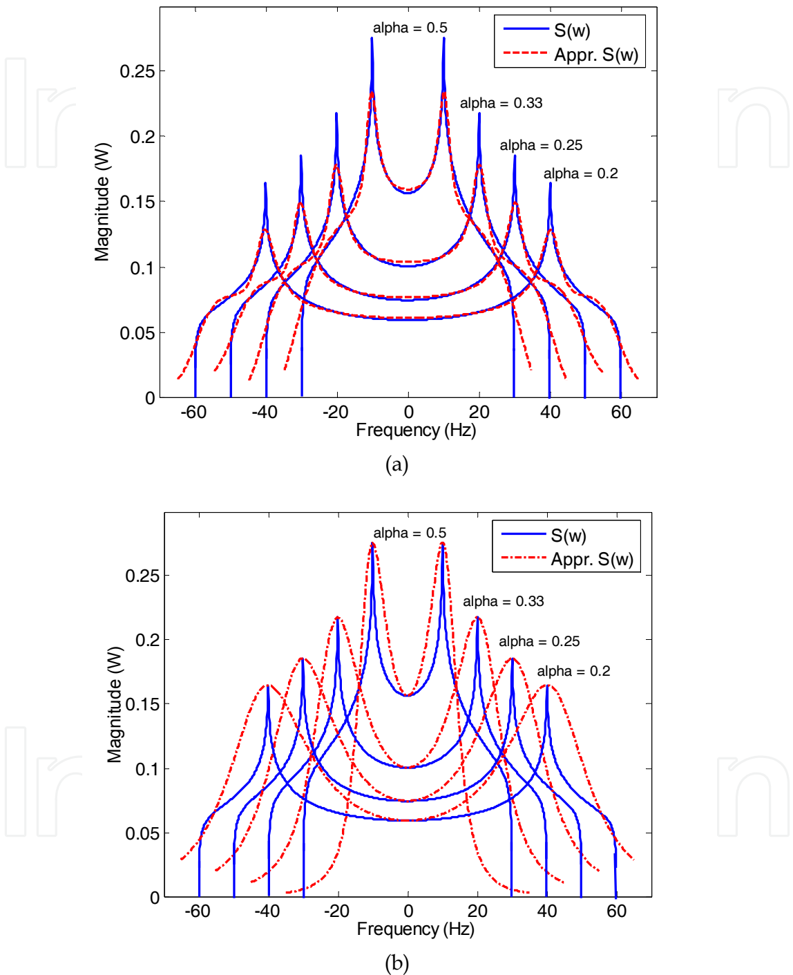
Fig. 12. DPSD, S(f) , and its approximation, \tilde{S}(f) , via 4 th order function for different \alpha 's using (a) the complex cepstrum, and (b) the simple approximation methods.
