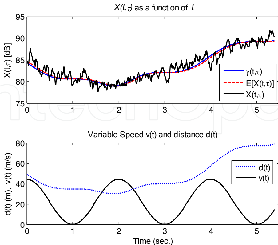
Fig. 3. Mean-reverting power path-loss X(t, \tau) for the TV LTF wireless channel model in Example 2.
