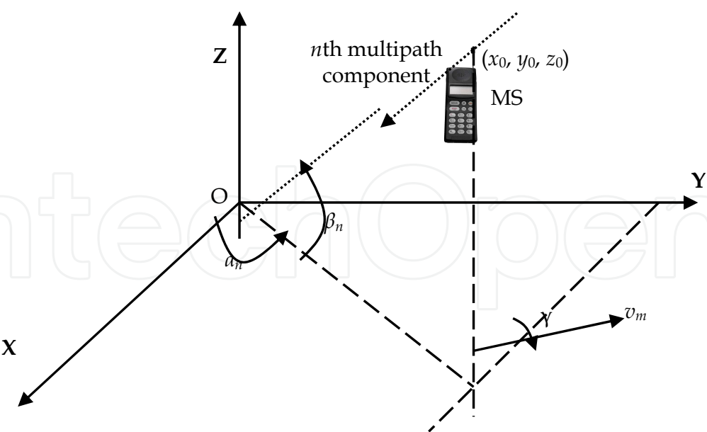
Fig. 4. Aulin’s 3D multipath channel model.
