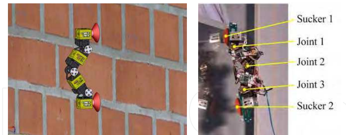
Fig. 4. Robotic inchworm design in CAD and real prototype
